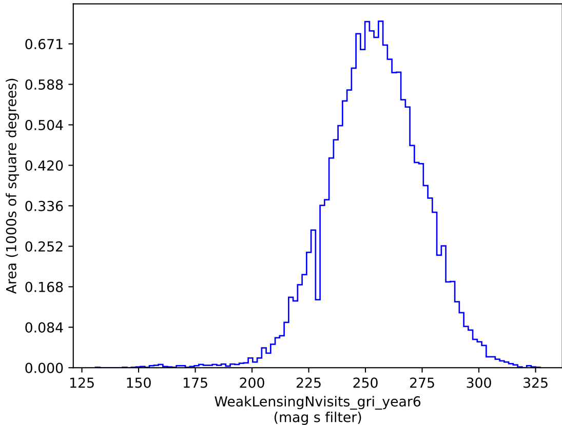
baseline_v3.2_10yrs gri band non-DD: WeakLensingNvisits_gri_year6
