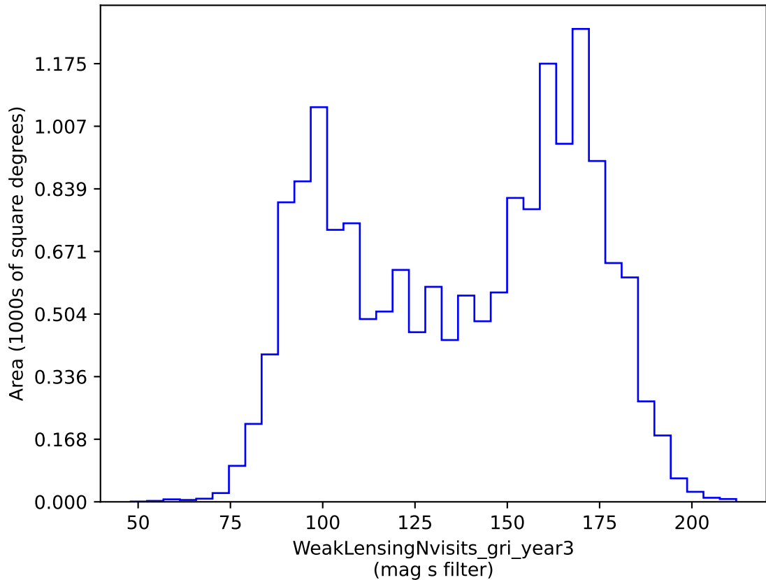
baseline_v3.2_10yrs gri band non-DD: WeakLensingNvisits_gri_year3
