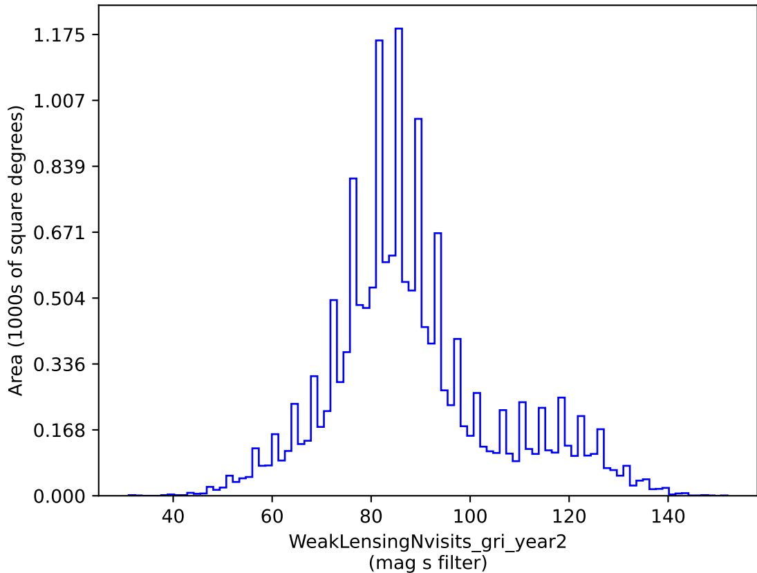
baseline_v3.2_10yrs gri band non-DD: WeakLensingNvisits_gri_year2
