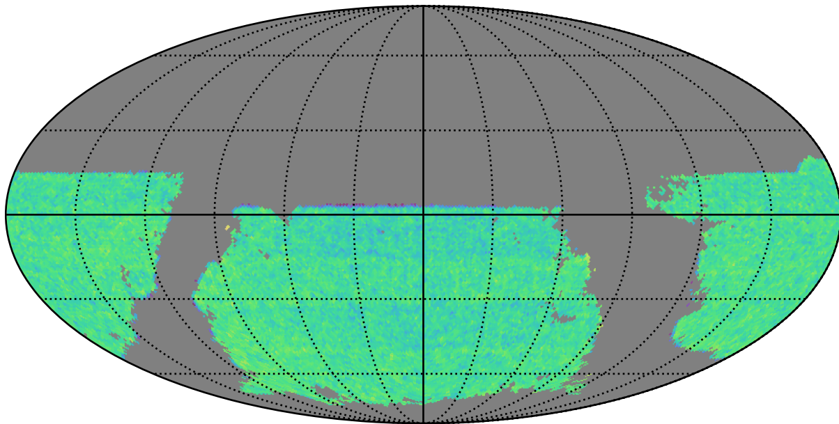
baseline_v3.2_10yrs gri band non-DD: WeakLensingNvisits
