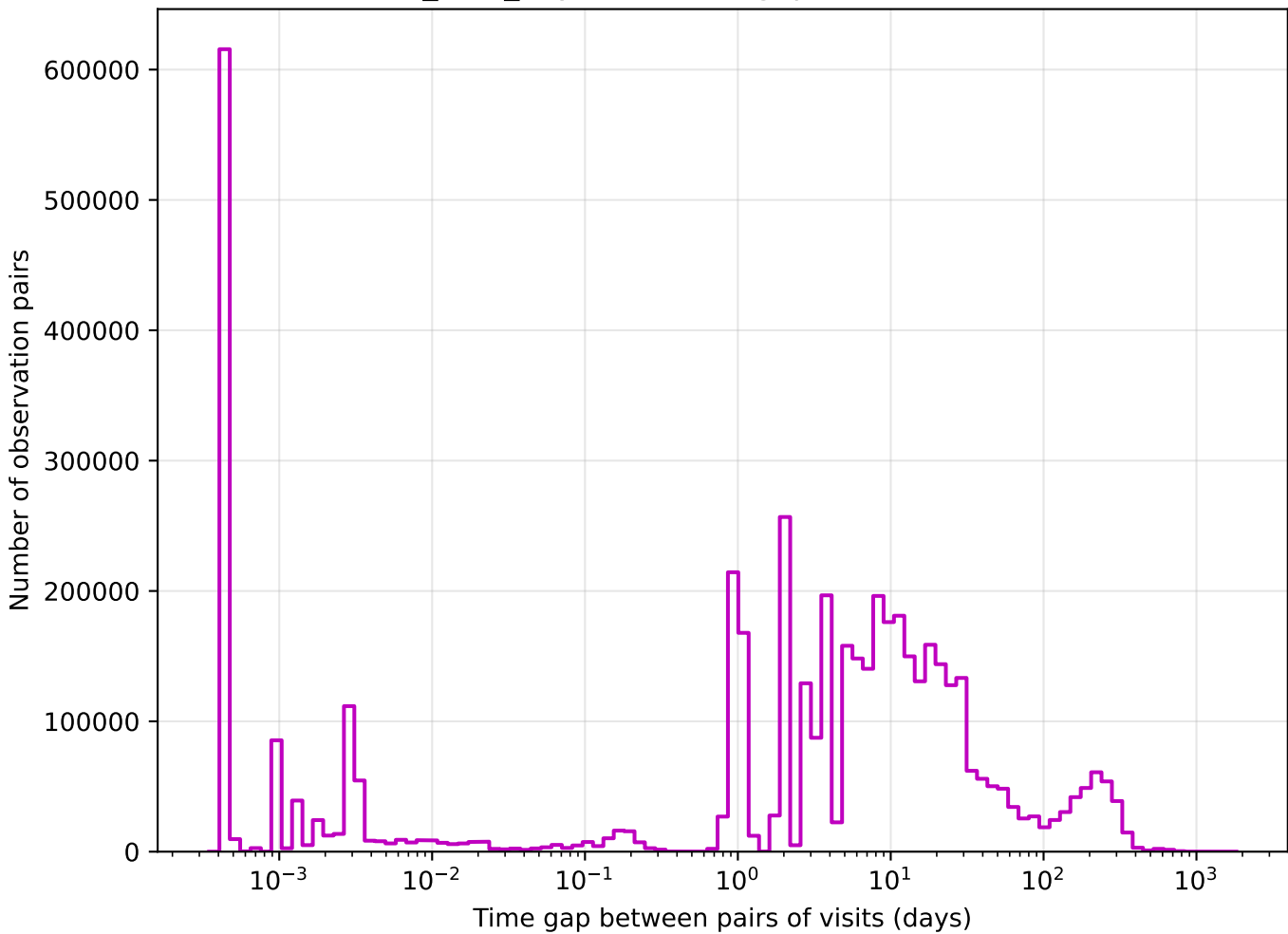
baseline_v3.2_10yrs z band: Tgaps observationStartMJD
