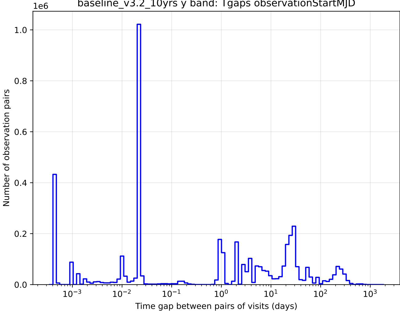
baseline_v3.2_10yrs y band: Tgaps observationStartMJD
