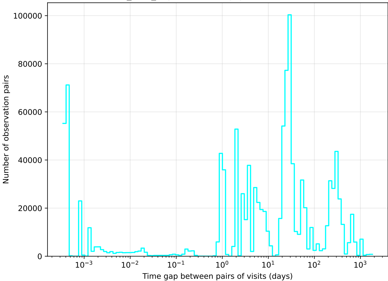
baseline_v3.2_10yrs u band: Tgaps observationStartMJD
