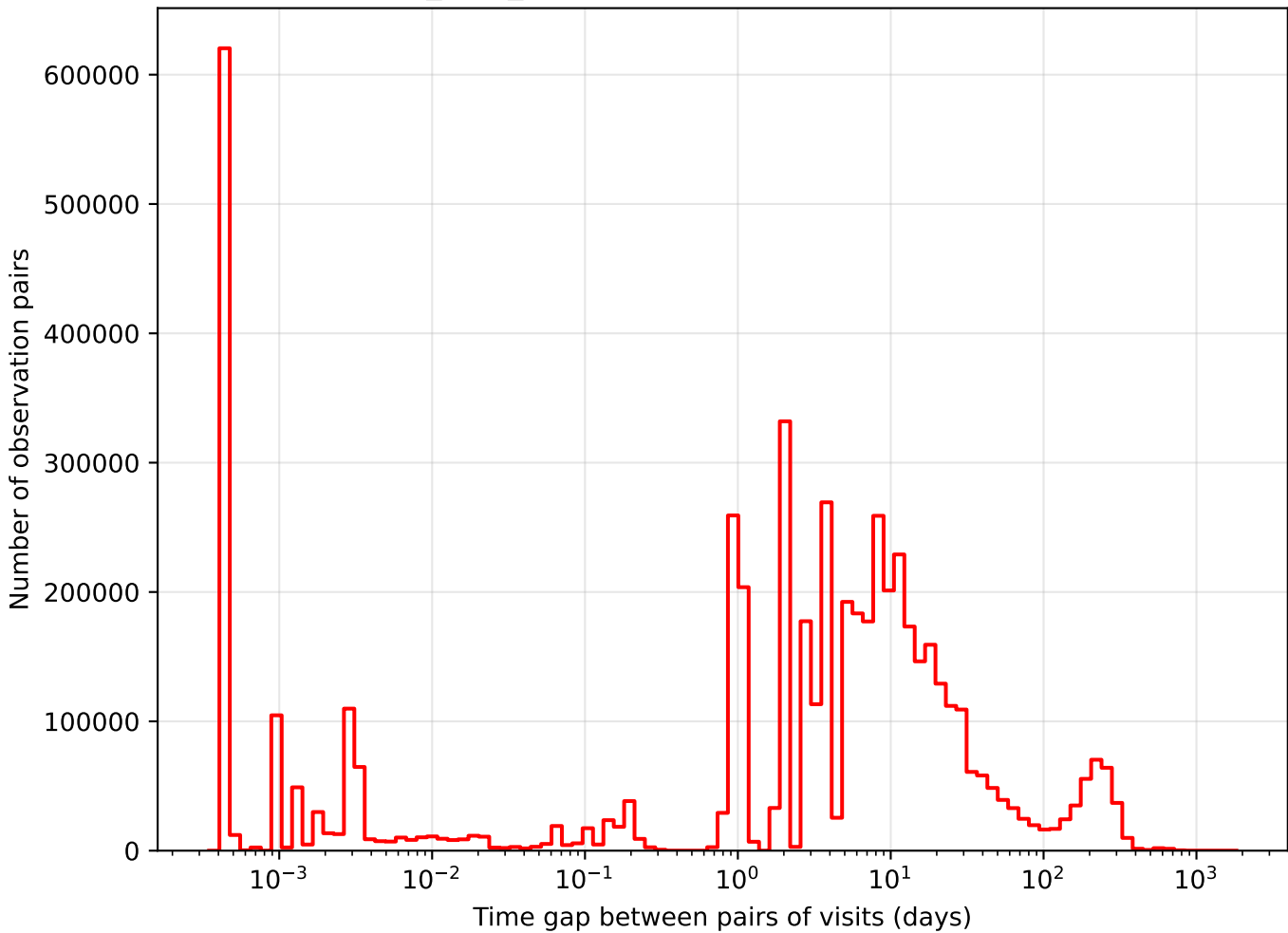
baseline_v3.2_10yrs i band: Tgaps observationStartMJD
