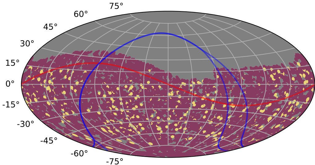
baseline_v3.2_10yrs : TDEsPopMetric_some_color
