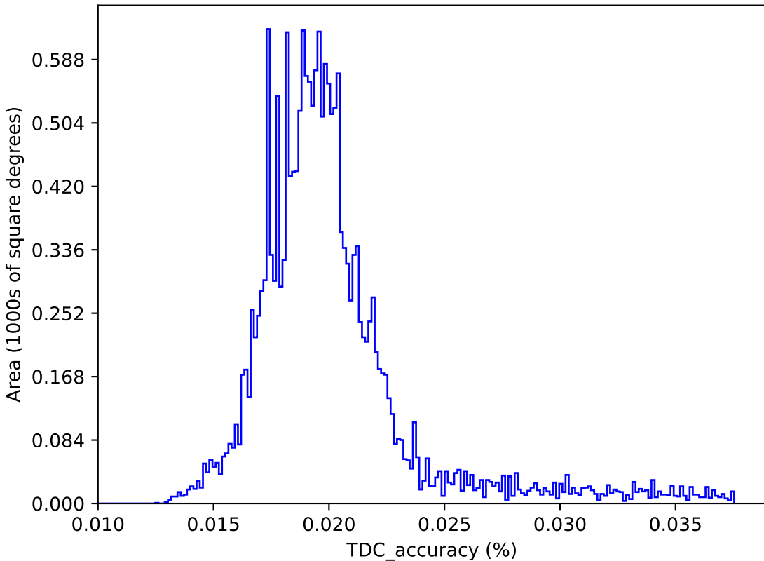
baseline_v3.2_10yrs : TDC_accuracy
