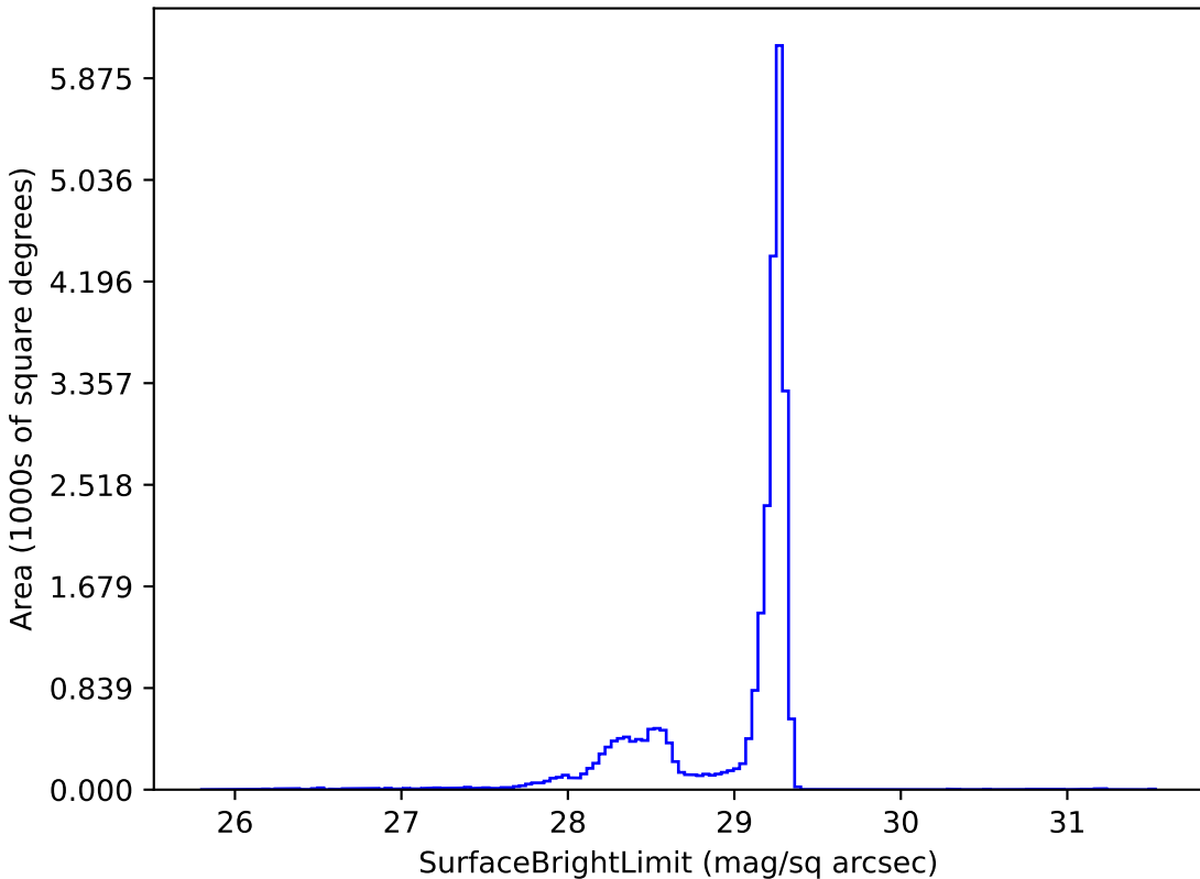
baseline_v3.2_10yrs z: SurfaceBrightLimit
