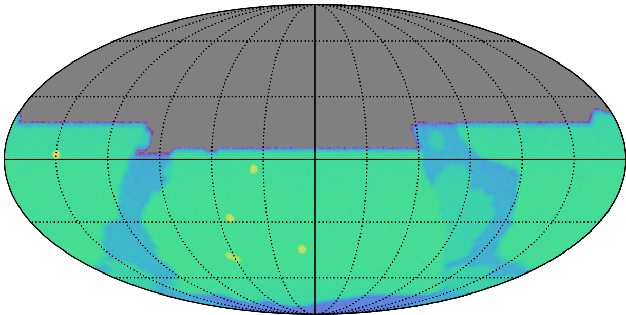
baseline_v3.2_10yrs y: SurfaceBrightLimit
