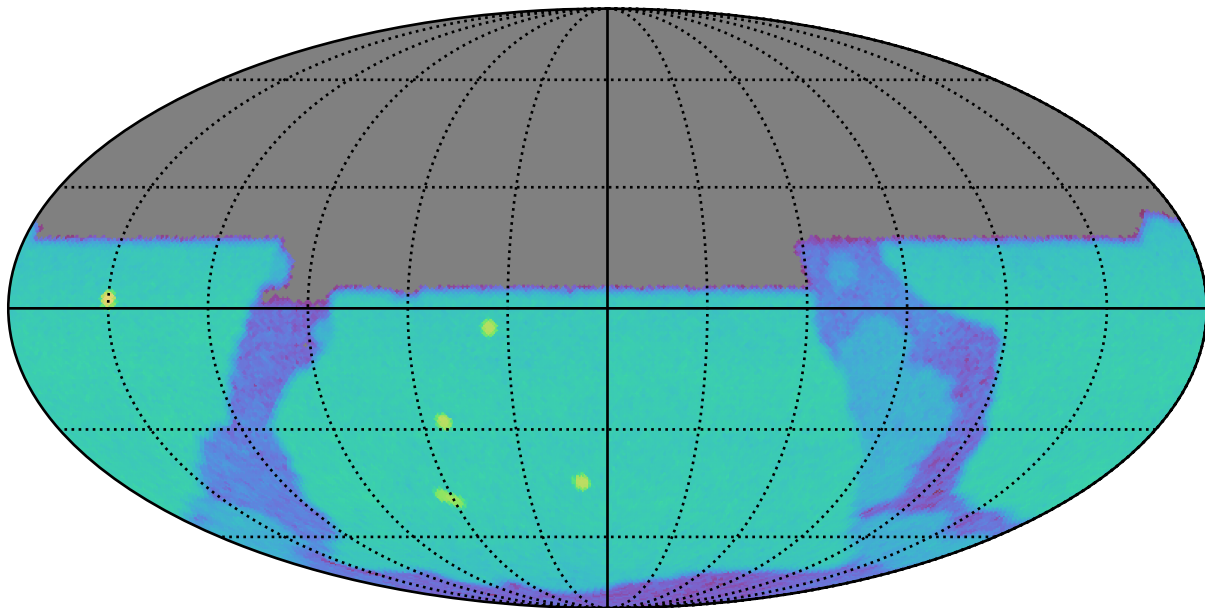
baseline_v3.2_10yrs u: SurfaceBrightLimit
