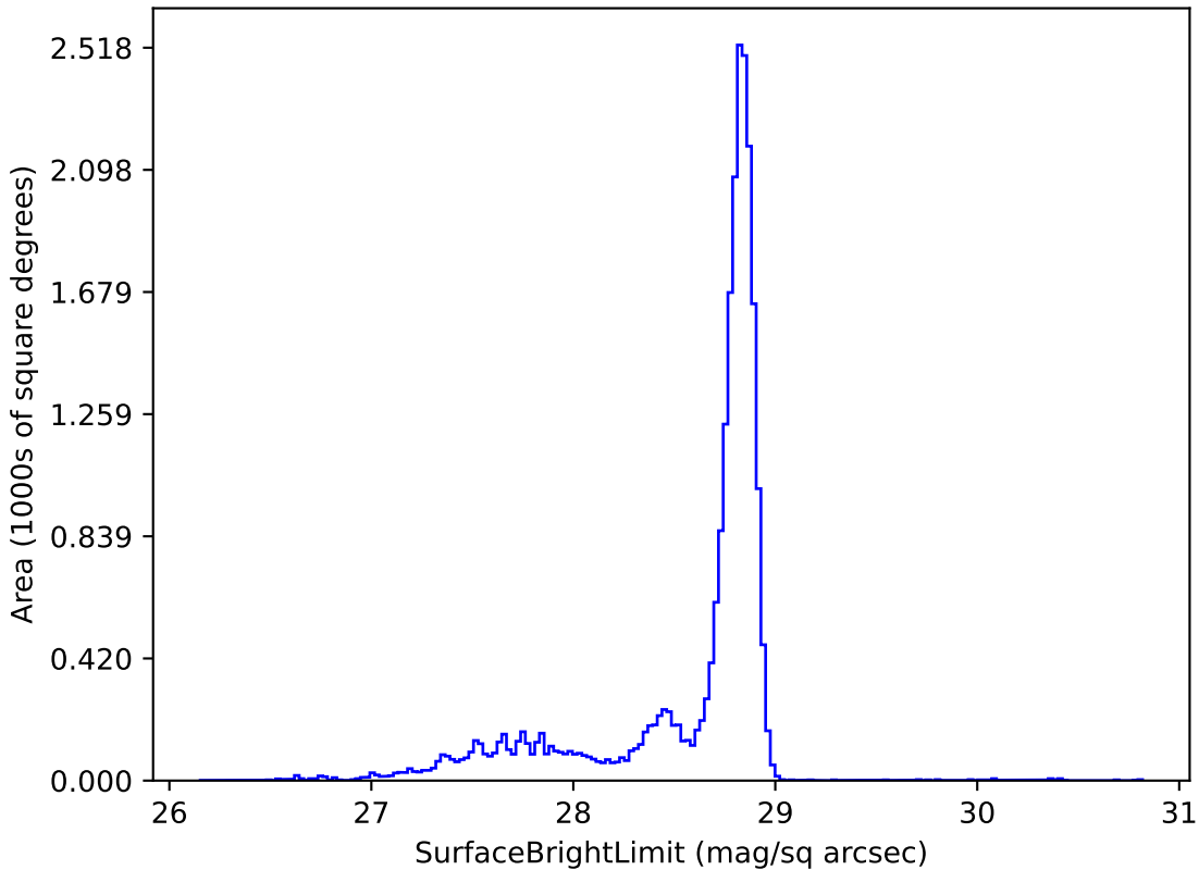
baseline_v3.2_10yrs u: SurfaceBrightLimit
