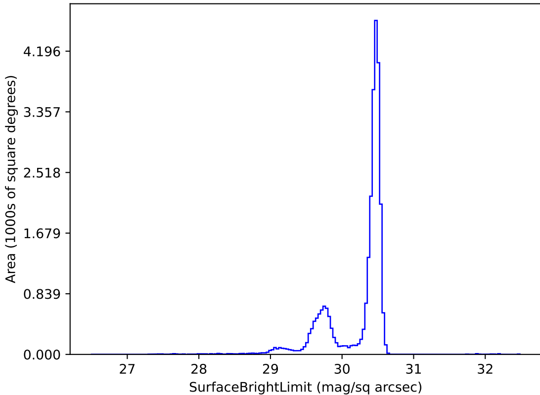
baseline_v3.2_10yrs r: SurfaceBrightLimit
