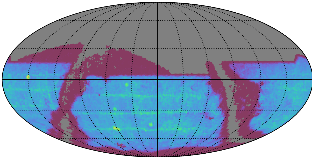
baseline_v3.2_10yrs : SNSLMetric
