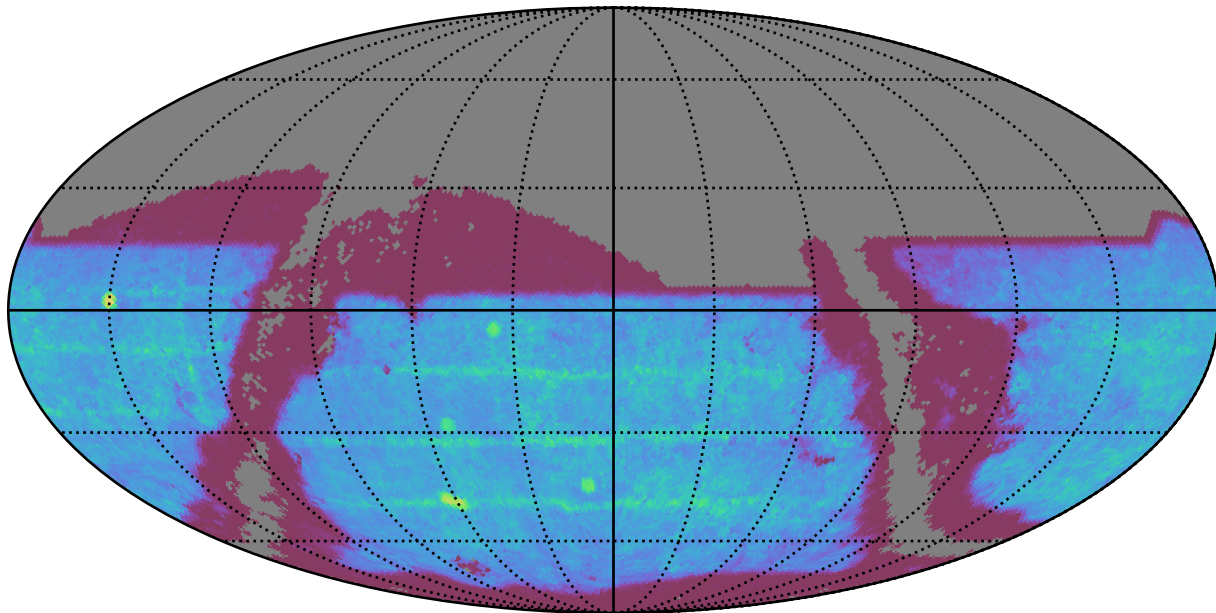
baseline_v3.2_10yrs : SNSLMetric
