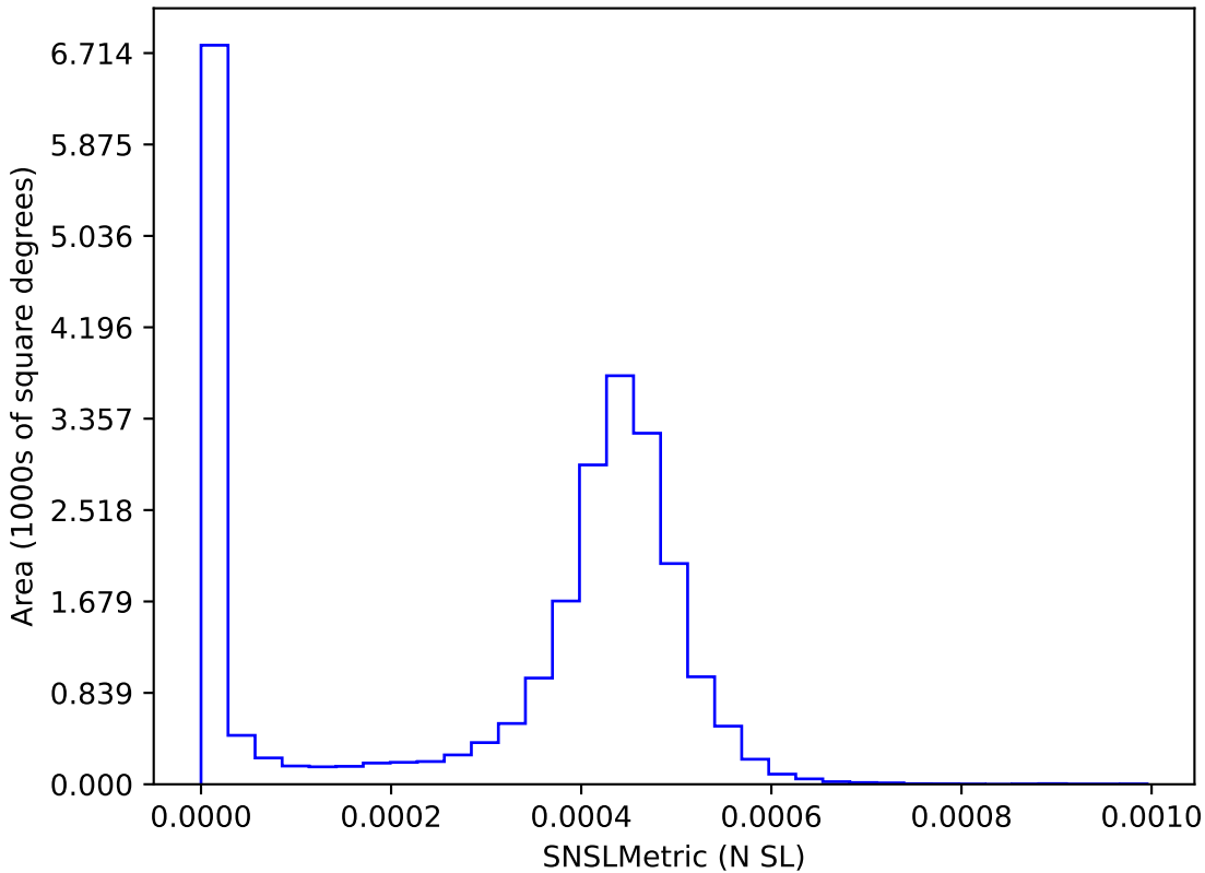
baseline_v3.2_10yrs : SNSLMetric
