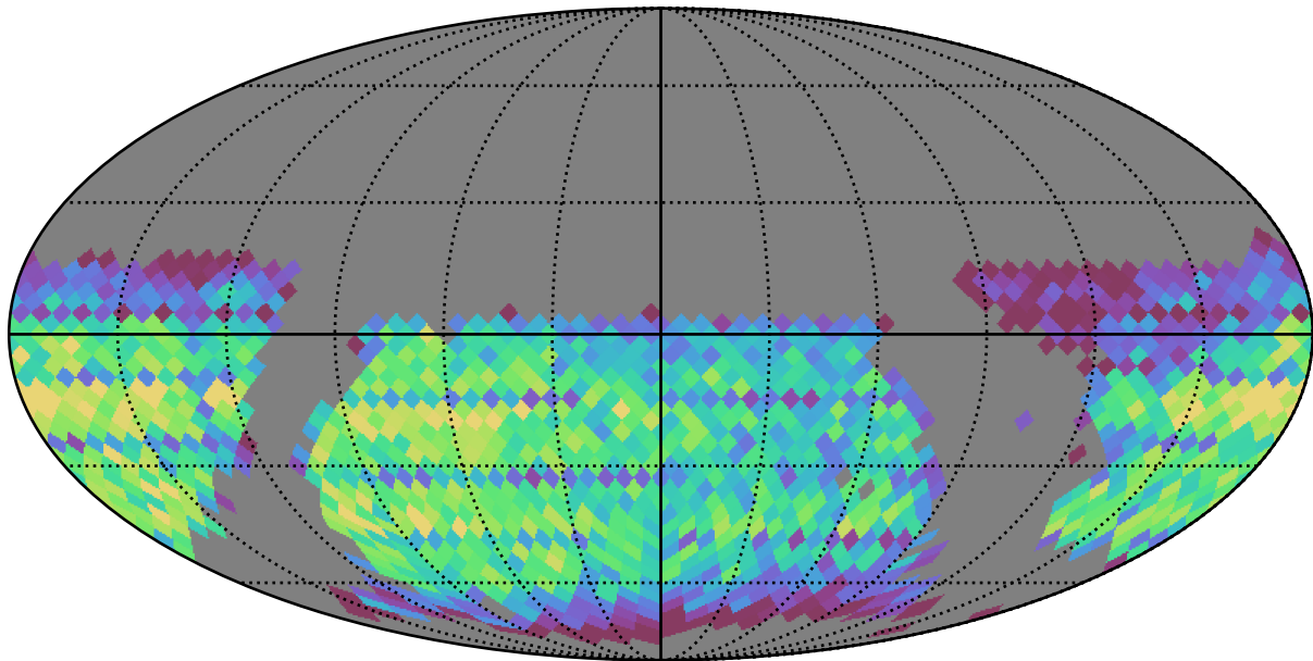
baseline_v3.2_10yrs DDF excluded: SNNSNMetric_reducezlim
