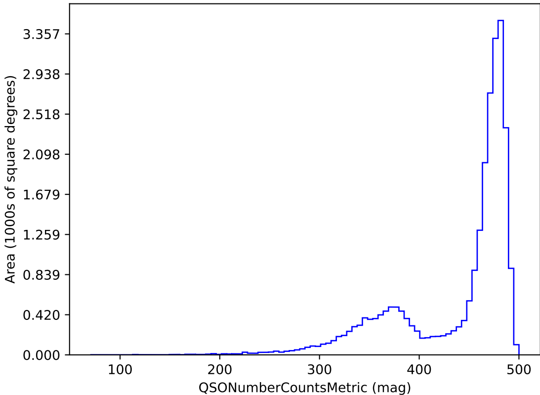
baseline_v3.2_10yrs z band and non-DD: QSONumberCountsMetric
