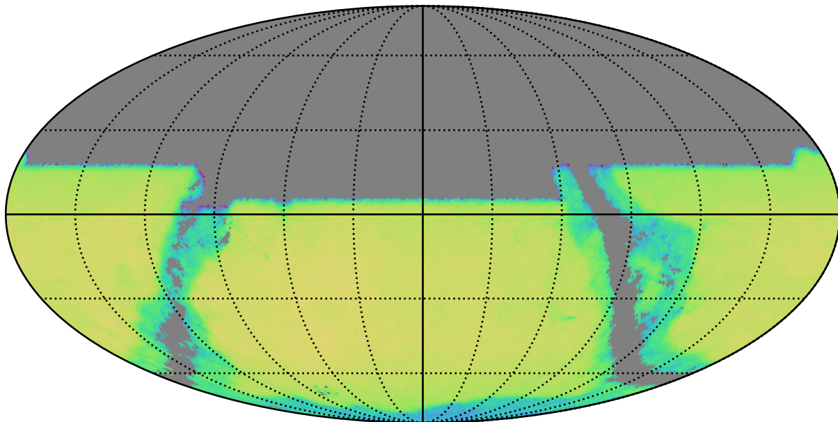
baseline_v3.2_10yrs y band and non-DD: QSONumberCountsMetric
