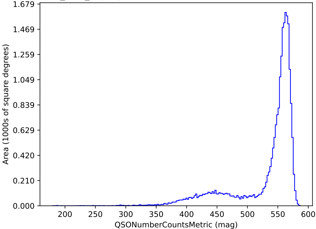
baseline_v3.2_10yrs y band and non-DD: QSONumberCountsMetric
