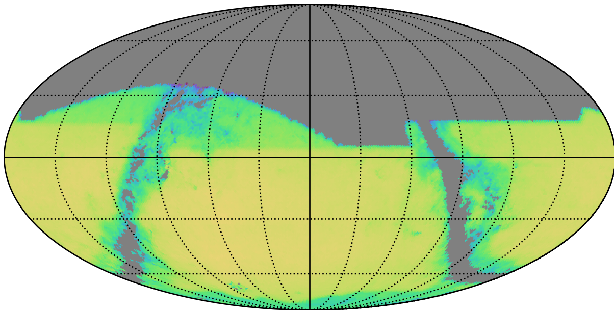
baseline_v3.2_10yrs r band and non-DD: QSONumberCountsMetric
