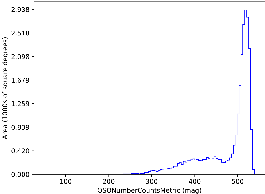
baseline_v3.2_10yrs r band and non-DD: QSONumberCountsMetric
