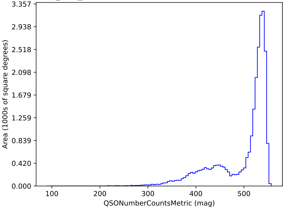
baseline_v3.2_10yrs i band and non-DD: QSONumberCountsMetric
