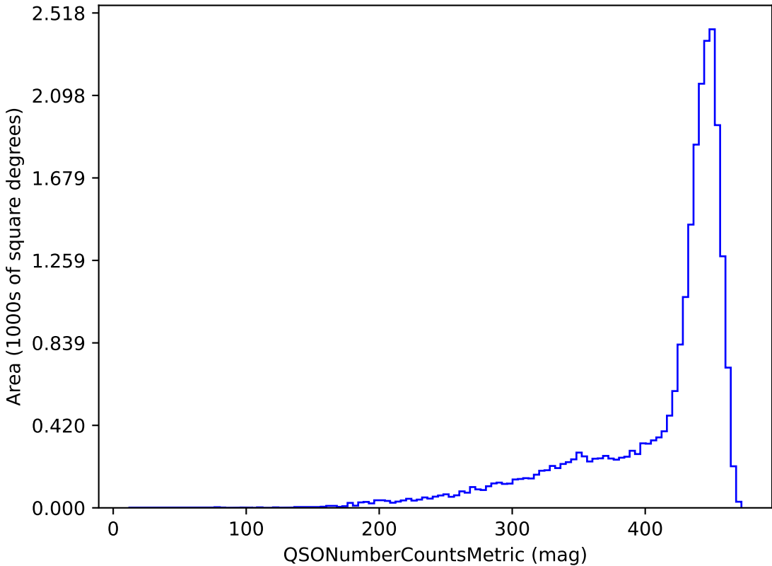
baseline_v3.2_10yrs g band and non-DD: QSONumberCountsMetric
