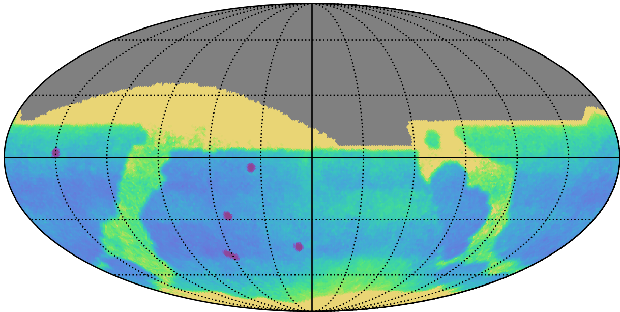
baseline_v3.2_10yrs : Proper Motion Uncert @ 24.0
