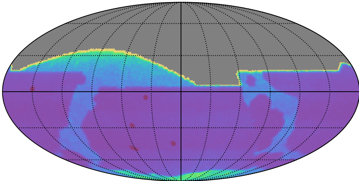
baseline_v3.2_10yrs : Proper Motion Uncert @ 20.5
