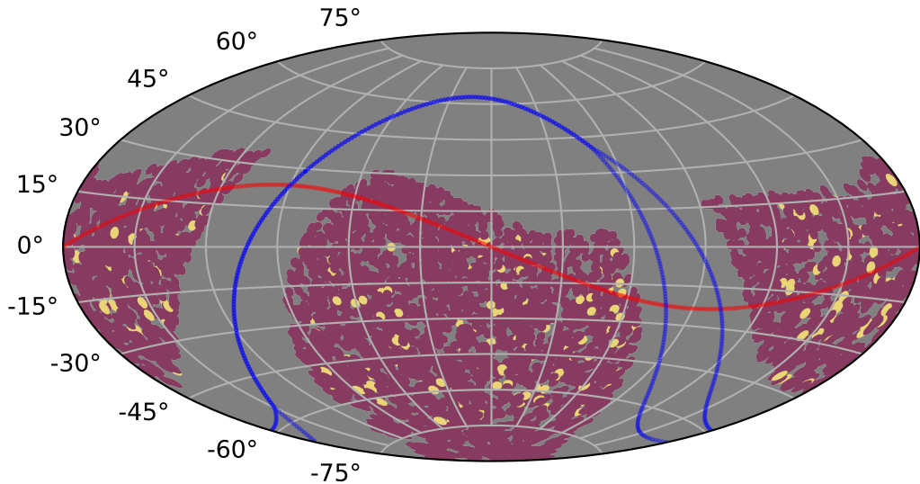
baseline_v3.2_10yrs : PrestoKNe_score_s
