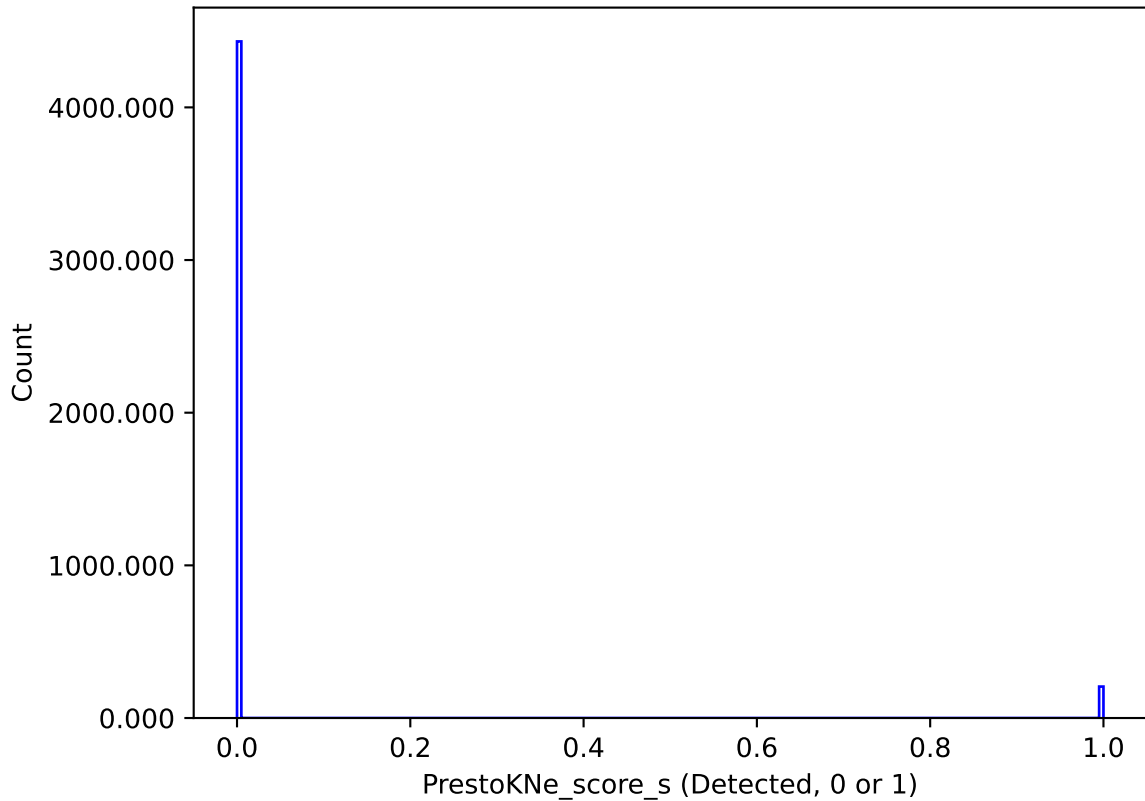
baseline_v3.2_10yrs : PrestoKNe_score_s
