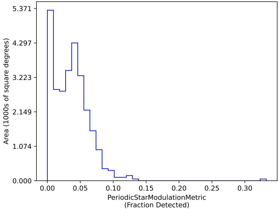
baseline_v3.2_10yrs dm 21 interval 30 RRc Year 1-2: PeriodicStarModulationMetric
