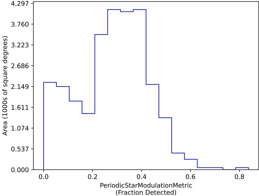
baseline_v3.2_10yrs dm 19 interval 30 RRc Year 1-2: PeriodicStarModulationMetric
