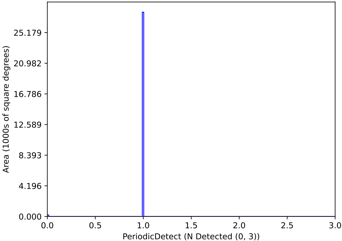
baseline_v3.2_10yrs P_2.0_Mag_24_Amp_0.05-0.1-1: PeriodicDetect
