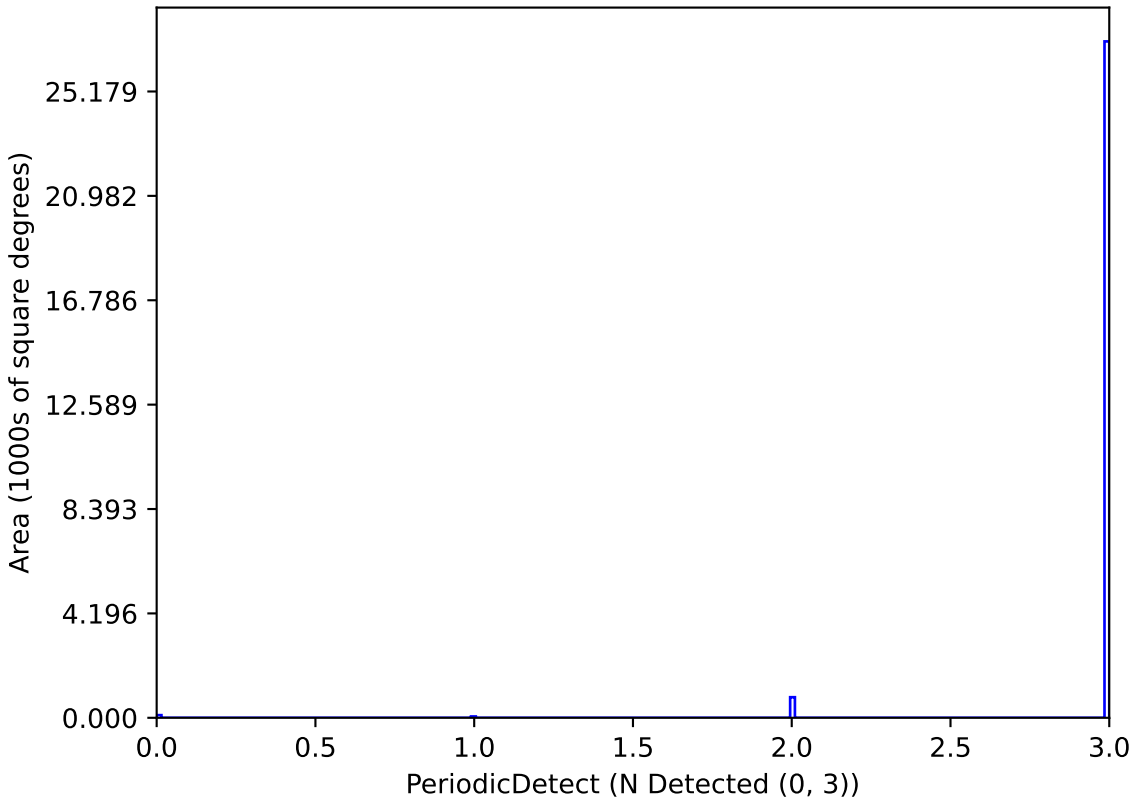
baseline_v3.2_10yrs P_2.0_Mag_21_Amp_0.05-0.1-1: PeriodicDetect
