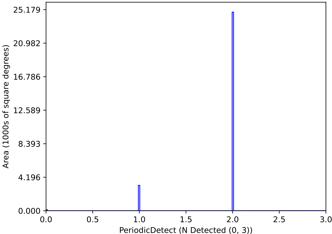
baseline_v3.2_10yrs P_1.0_Mag_21_Amp_0.05-0.1-1: PeriodicDetect
