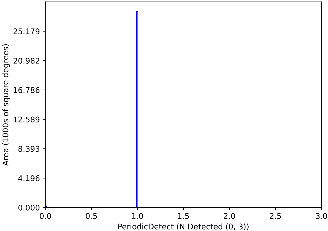
baseline_v3.2_10yrs P_0.5_Mag_24_Amp_0.05-0.1-1: PeriodicDetect
