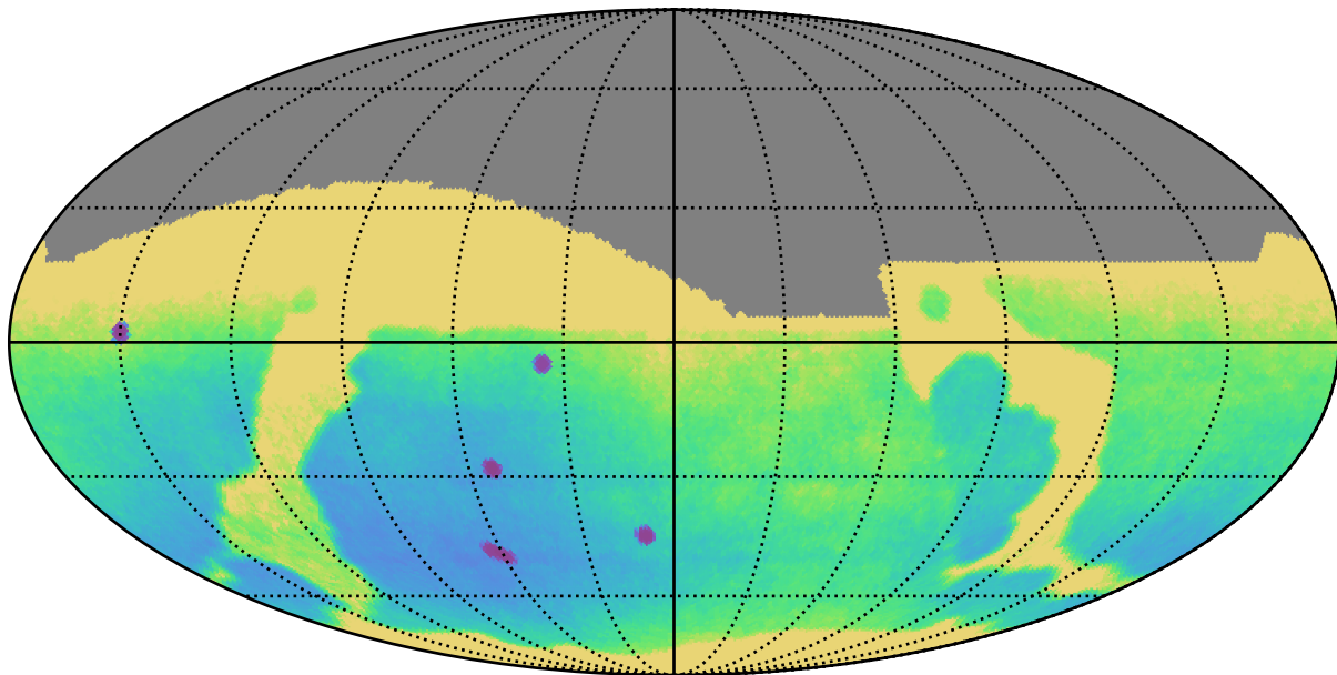
baseline_v3.2_10yrs : Parallax Uncert @ 24.0
