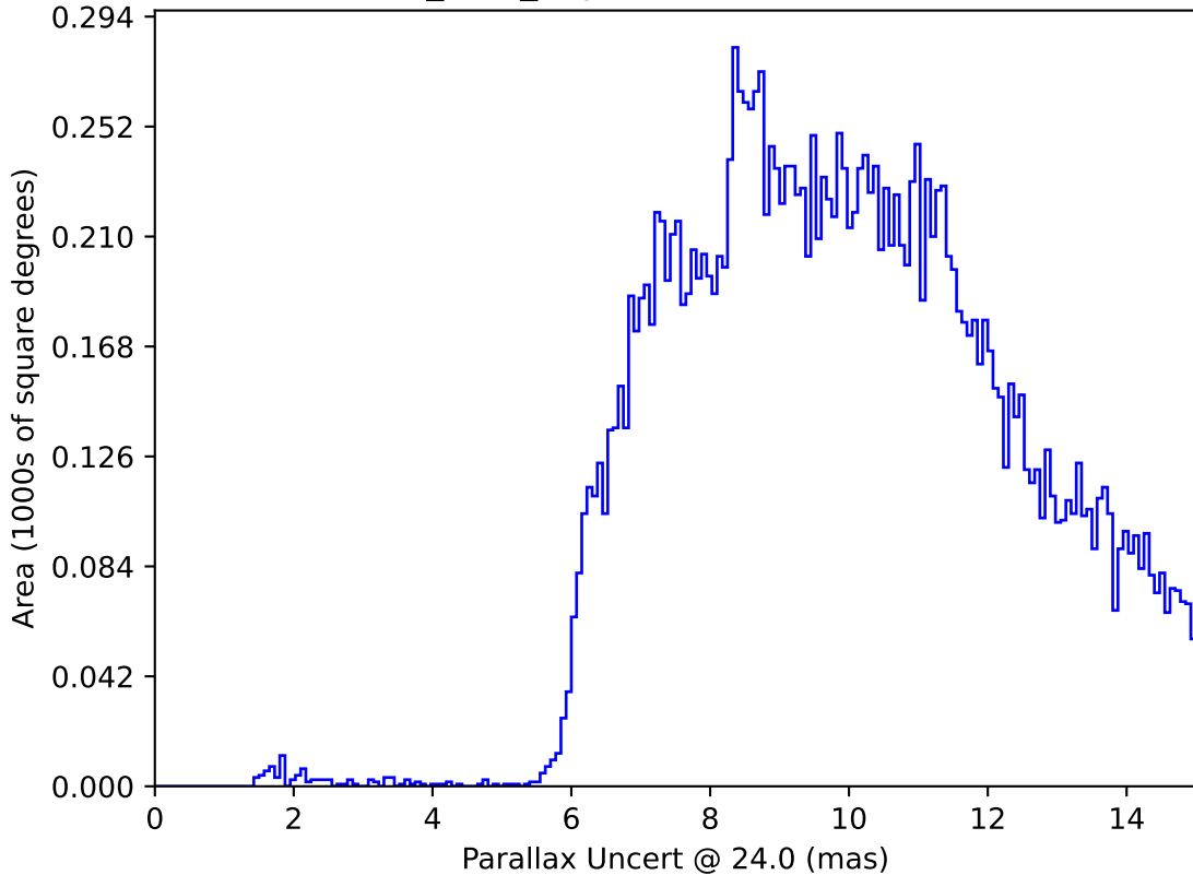
baseline_v3.2_10yrs : Parallax Uncert @ 24.0
