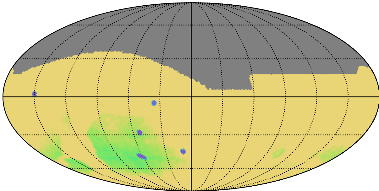
baseline_v3.2_10yrs : Parallax Uncert @ 22.4
