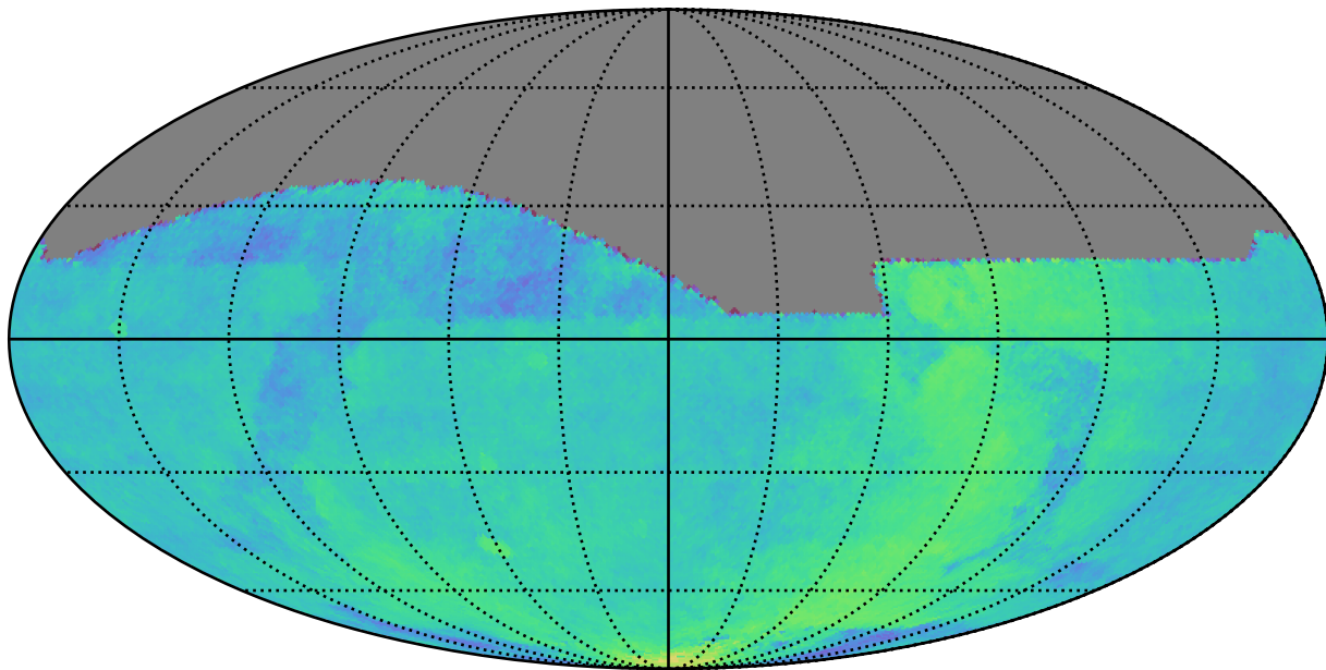
baseline_v3.2_10yrs : Parallax Coverage @ 22.4
