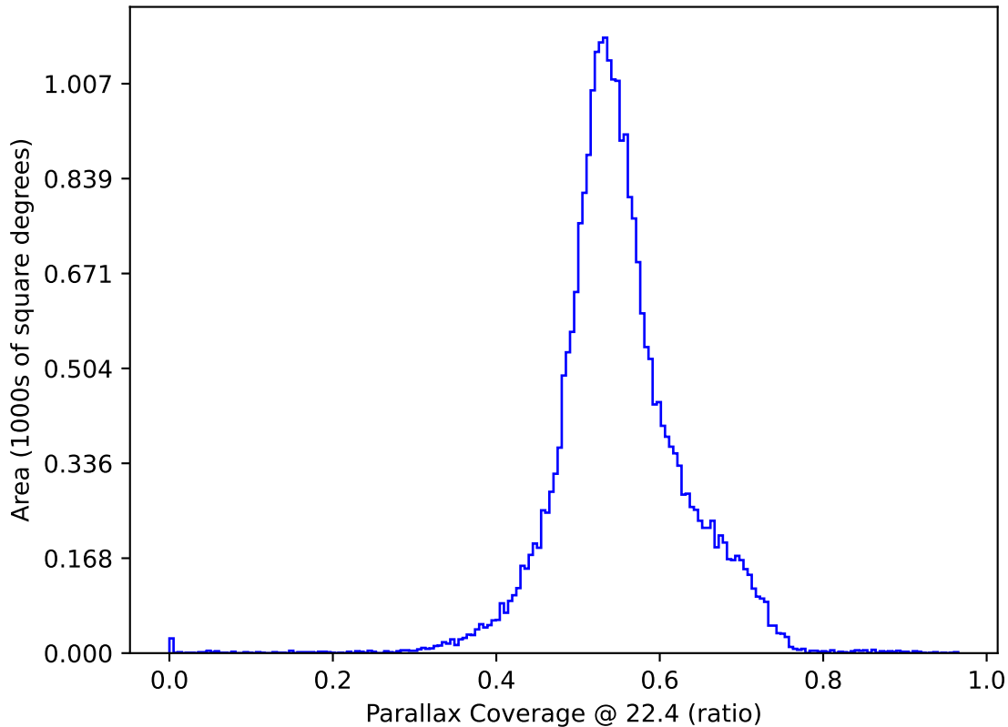
baseline_v3.2_10yrs : Parallax Coverage @ 22.4
