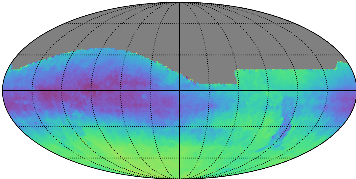
baseline_v3.2_10yrs : Parallax-DCR degeneracy @ 24.0
