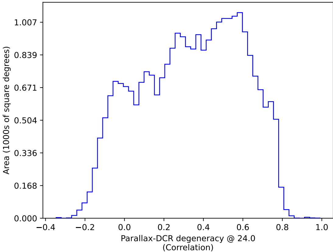
baseline_v3.2_10yrs : Parallax-DCR degeneracy @ 24.0
