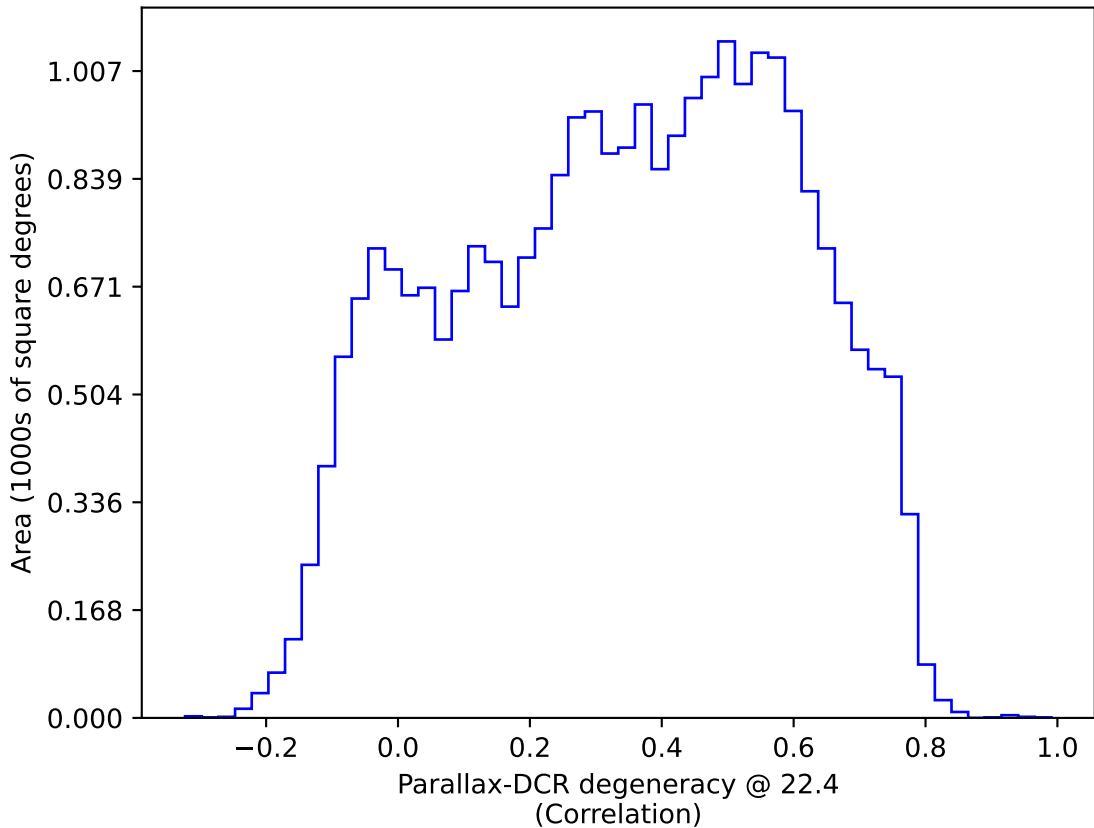
baseline_v3.2_10yrs : Parallax-DCR degeneracy @ 22.4
