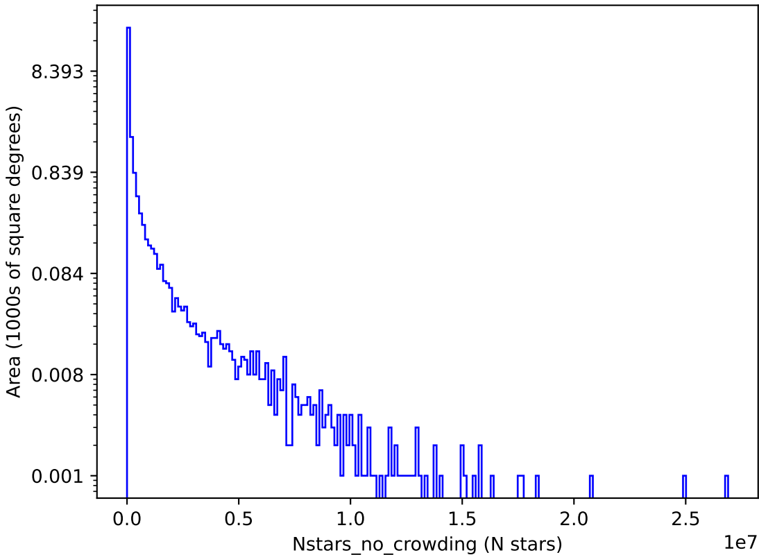
baseline_v3.2_10yrs z: Nstars_no_crowding
