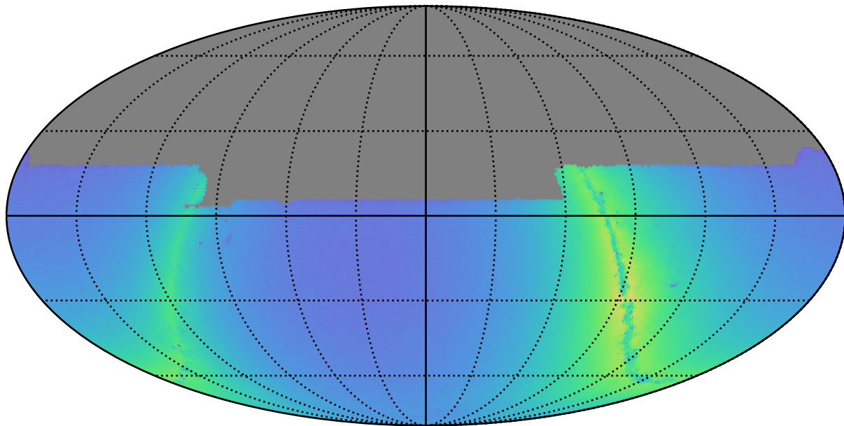
baseline_v3.2_10yrs y: Nstars_no_crowding
