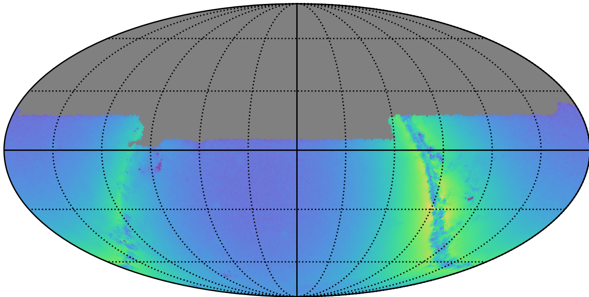
baseline_v3.2_10yrs u: Nstars_no_crowding
