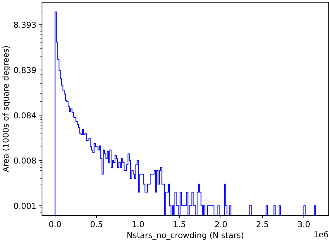
baseline_v3.2_10yrs u: Nstars_no_crowding
