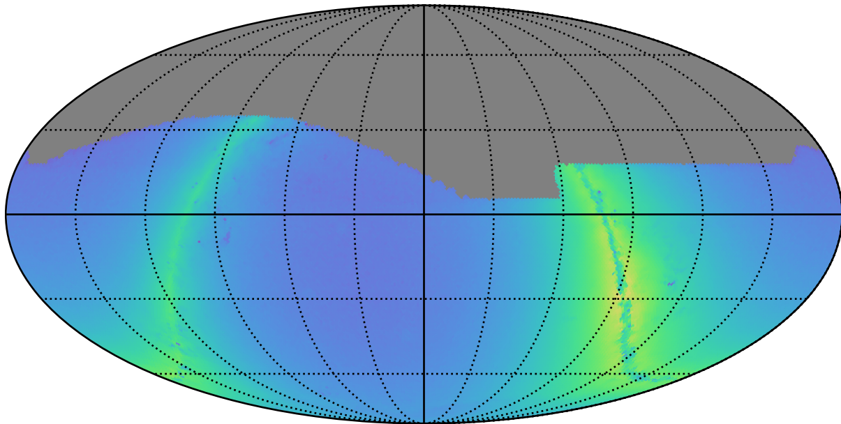
baseline_v3.2_10yrs r: Nstars_no_crowding
