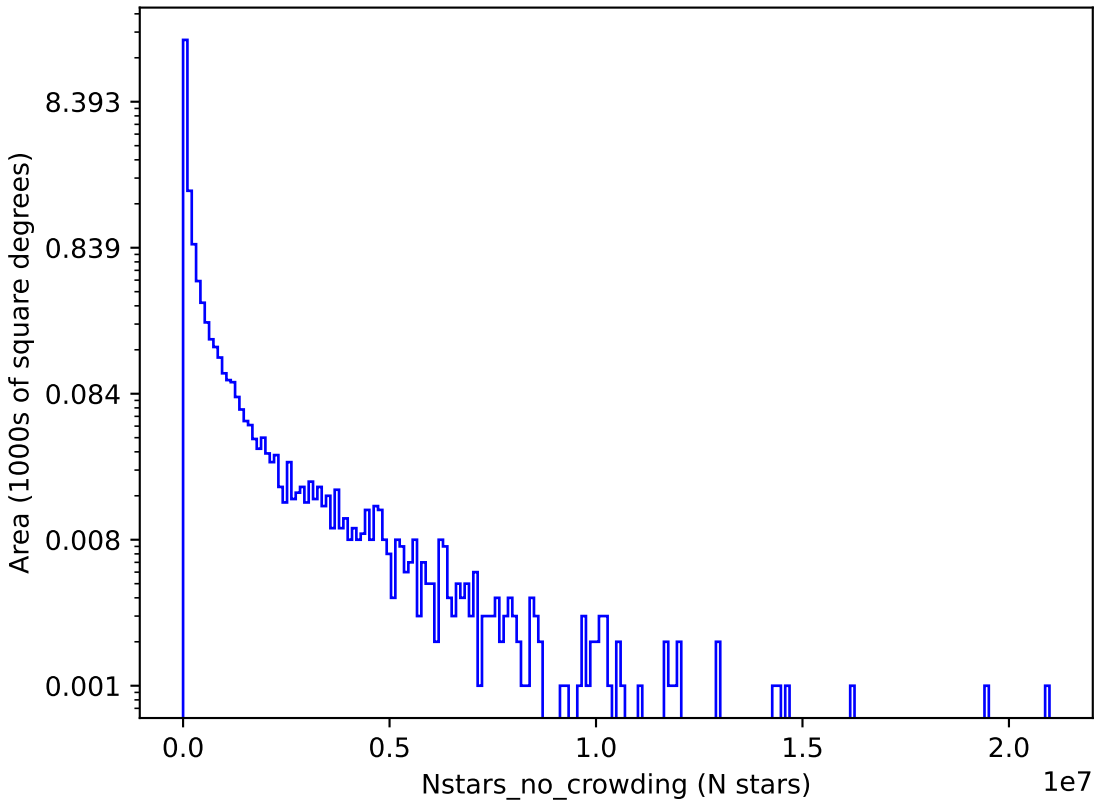
baseline_v3.2_10yrs r: Nstars_no_crowding
