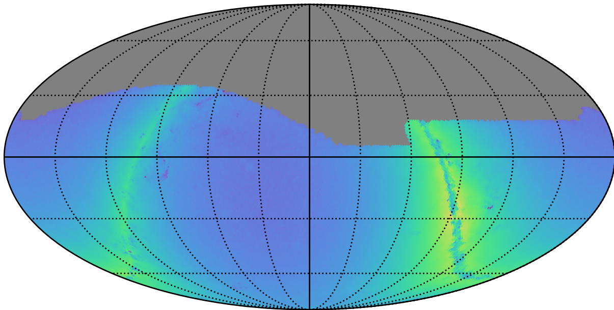
baseline_v3.2_10yrs g: Nstars_no_crowding
